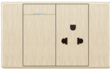
BLF4-K11FC 1 Gang 1Way switch and Philippines Socket BLF4-K22YCS 1 Gang 2Way switch and Philippines Socket 15A 110/250V
