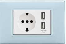
BLFS-DCUSB 2Usb and Germany Socket 16A 250V
