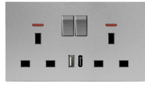
BLW1S-YF2SUSBC 2X13A switched socket+USB+ Type-C neon SP BLW1S-YF2DUSBC 2X13A switched socket+USB+ Type-C neon DP
